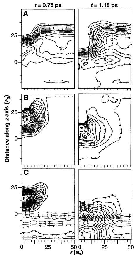
Fig. 4. Contours of (A) density ( \rho ), (B) temperature ( T ), and (C) pressure ( P ) of the target surface (initially at T = 40 K) recorded at t = 0.75 ps (left column) and t = 1.15 ps (right column) during the deposition of a (\text{NaCl})_{32} nanocrystal (Ne I orientation) on a Ne film adsorbed on a NaCl crystal. The origin of the z axis (normal to surface) is at the average location of the topmost layer of the crystalline NaCl substrate. The average thickness of the film is 31 a_0 . In the calculation of the contours of a property at any given region, the value was weighted by a Gaussian of width 3a_0 ( \delta ). Tick marks on contour lines point in the direction of increase in the value. The increment between neighboring contours is \Delta_\rho = 5 \times 10^{-4} a_0^{-3} , \Delta_T = 94 K, and \Delta_P = 0.29 GPa, and the indicated values associated with selected contours are in units of 10^{-3} a_0^{-3} , 10^3 K, and gigapascals for \rho , T , and P , respectively. Note the formation of a crater in the fluid caused by the incoming cluster. Fluid particles propagate down toward the solid substrate and sideways in the film, leading to densification and bulging of the fluid (A). The pressure and temperature impulses propagate down and expand radially, transmitting at the latter time into the underlying solid substrate (B and C).
