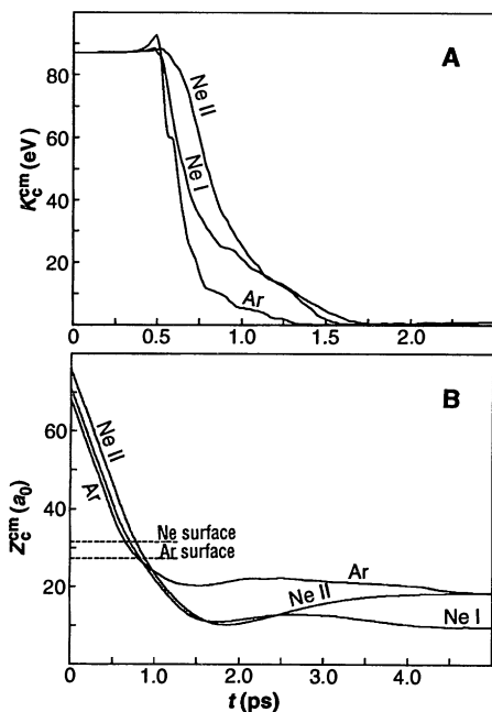
Fig. 1. (A) Kinetic energy and (B) center-of-mass position (on z axis) of a (\text{NaCl})_{32} nano-cluster incident on adsorbed liquid Ar or Ne films plotted versus time. For the Ne film, two initial orientations, Ne I and Ne II, correspond to cubic clusters impinging with the face or corner of the cube, respectively, directed toward the target surface. The origin of the distance axis in (B) is at the average location of atoms in the topmost layer of the underlying crystalline NaCl substrate. The average locations of the top of the liquid films are indicated.
