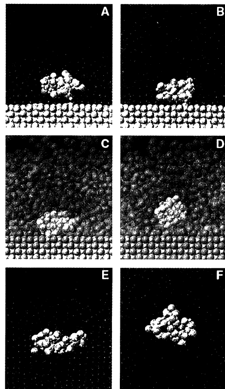
Fig. 3. Selected atomic configurations from simulations of collisions of an initially ordered NaCl nanocrystal (Na, yellow; Cl, green) with adsorbed Ar (red) and Ne (blue) fluids. Disordered (glassy) (\text{NaCl})_{32} cluster at (A) t = 2 ps and (B) t = 8 ps in collision with an Ar film. Ordered clusters, from the limiting cases of initial orientation (C) Ne I and (D) Ne II, soft landed on a Ne film ( t = 5 ps). The structural defect in (C) was caused by the initial impact with the liquid surface. Glassy nanocluster configurations, at (E) t = 2 ps and (F) t = 22 ps, formed in a higher energy collision (center-of-mass velocity of 4 \text{ km s}^{-1} ) with a thick Ar film (only a portion of the system surrounding the cluster is shown). Note the "porous" structure of the fluid in (F). In all cases, the structures of the clusters at longer times remain virtually the same as the ones shown.
