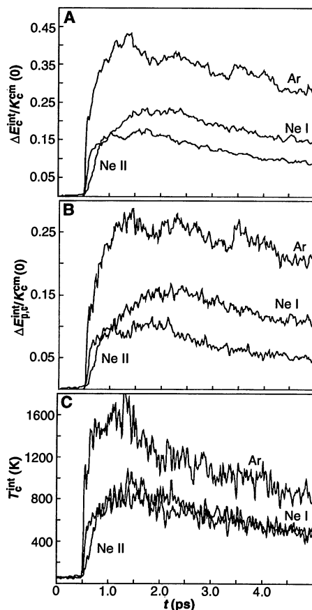
Fig. 2. Time evolution of the changes in (A) total internal energy and (B) internal potential energy from the average initial values for a (\text{NaCl})_{32} cluster colliding with liquid Ar or Ne films (Ne I and Ne II as in Fig. 1), plotted relative to the initial total incident translational energy of the cluster [ K_c^{\text{cm}}(0) = 87 eV]. (C) The corresponding variations with time of the internal kinetic temperature of the cluster.
