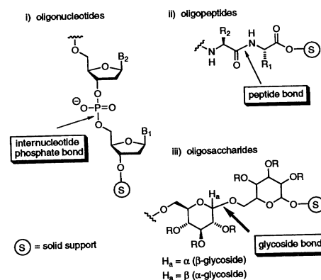
Fig. 1. Solid-phase synthesis of biopolymers.
