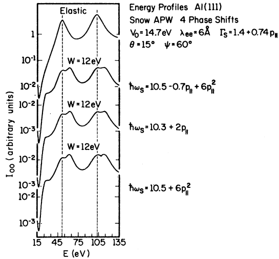
FIG. 1. Elastic ( w = 0 ) and w = 12 eV energy profiles for the (00) beam of electrons scattered from Al (111) associated with three dispersion relations the coefficients of which lie in the region of ambiguity (see, e.g., Fig. 4). A four-phase-shift two-step model was used with the values of the parameters indicated in the figure. Vertical dashed lines are drawn to guide the eye in locating the positions of the primary Bragg maxima.
